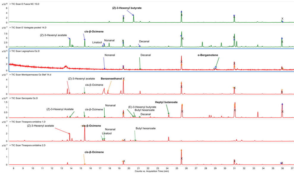
Figure 2 . Chromatograms from Erythrina plants from New Caledonia (in green from top to bottom: E. fusca , E. variegata ) and Menispermaceae plants from Australia (in red from top to bottom: Legnephora moorei , Stephania japonica , Sarcopetalum harveyanum , Tinospora smilacina (inland), Tinospora smilacina (coastal)) with most abundant compound in bold and the five compounds that triggered an electroantennogram responses across the two fruit piercing moth populations indicated for each plant. Peaks crossed are contaminants.
