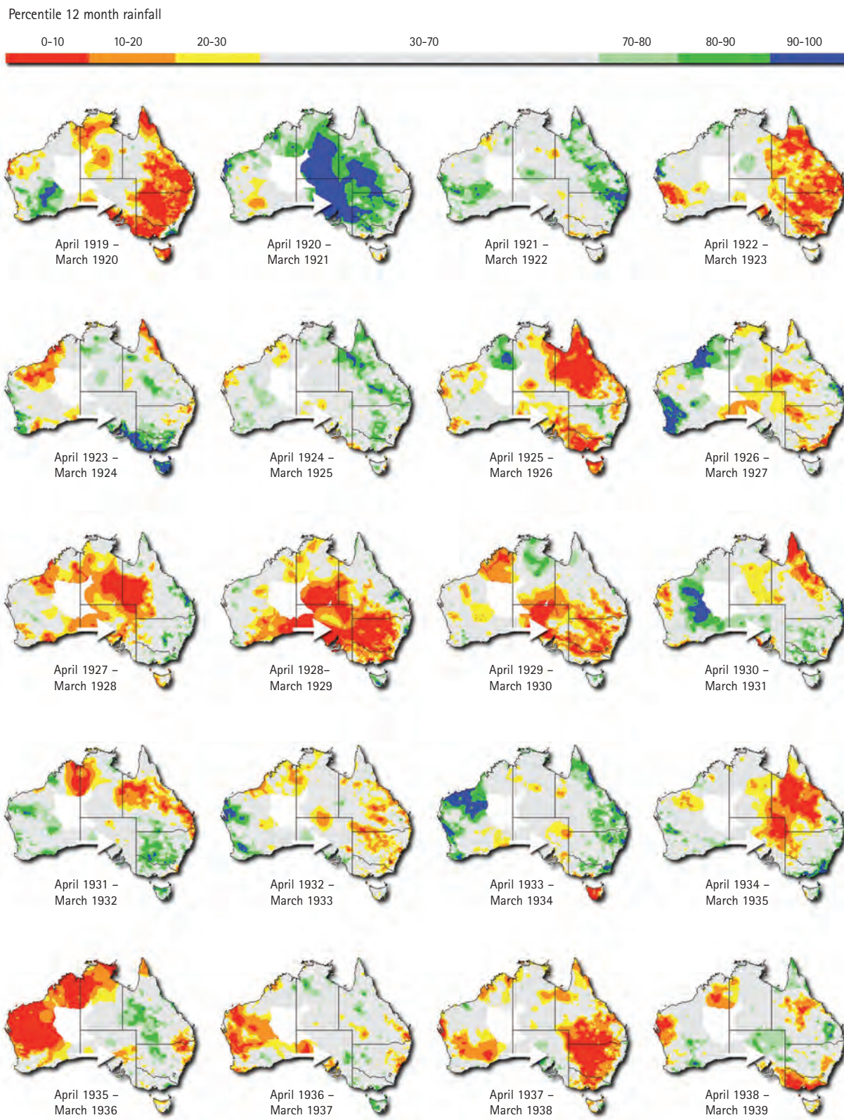
Plate 2.2 Rainfall (1 April to 31 March) expressed as a percentile over the last hundred years for Episode 2. The El Niño years were 1919/20, 1923/24, 1925/26, 1932/33. The La Niña years were 1921/22, 1924/25, 1938/39.
