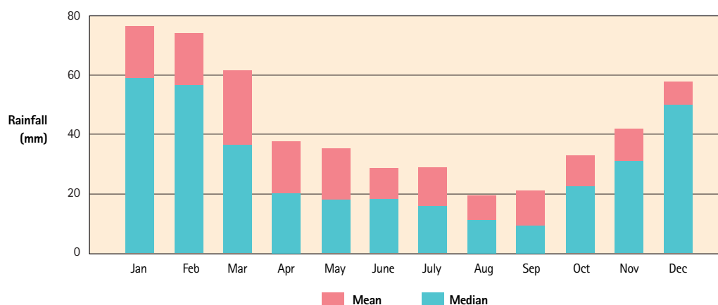
Figure 4.3. Mean and median monthly rainfall of Lansdowne for the period 1880–1998.
