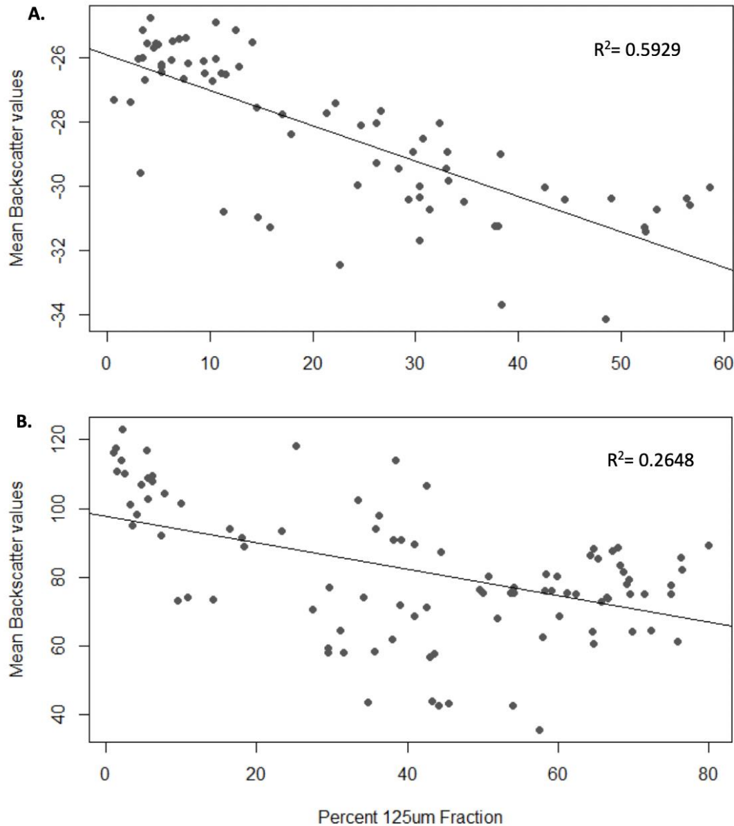
Figure 19-6. The relationship between mean backscatter values and 125 µm fraction in A) offshore from Gladstone ( R^2 = 0.5929 ) and, B) Hervey Bay ( R^2 = 0.2648 ). There is an inverse correlation between mean backscatter values and the 125 µm fraction in both locations.
