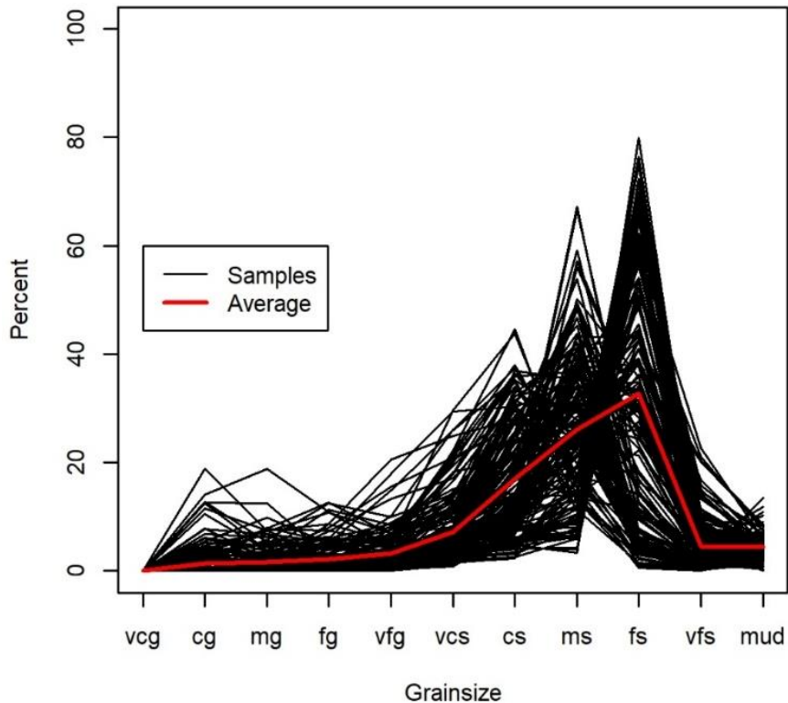
Figure 18-3. Histograms of the 166 sediment grainsize fractions based on the classification scheme of Table 18-1 and Wentworth (1922).
