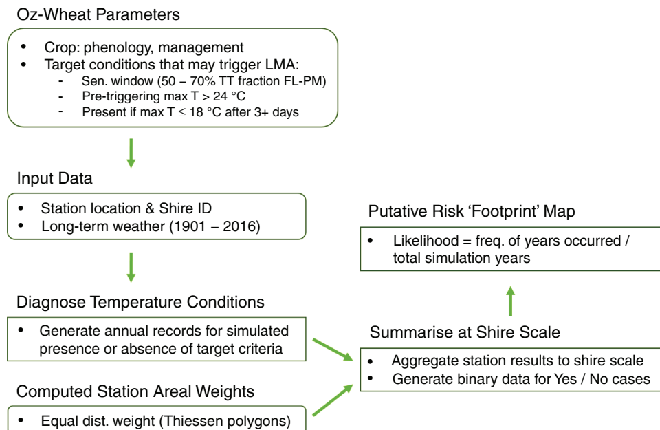
Fig. 2. Regional-scale analysis workflow applied for this study using Oz-Wheat modified for simulating one set of targeted temperature conditions similar to the cool-shock regime.
