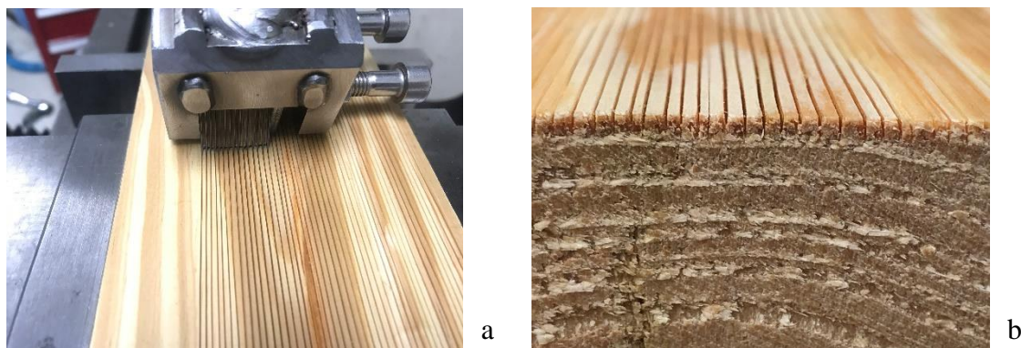
Fig. 1. Timber surface incised with special tool to a final depth of 2 mm
