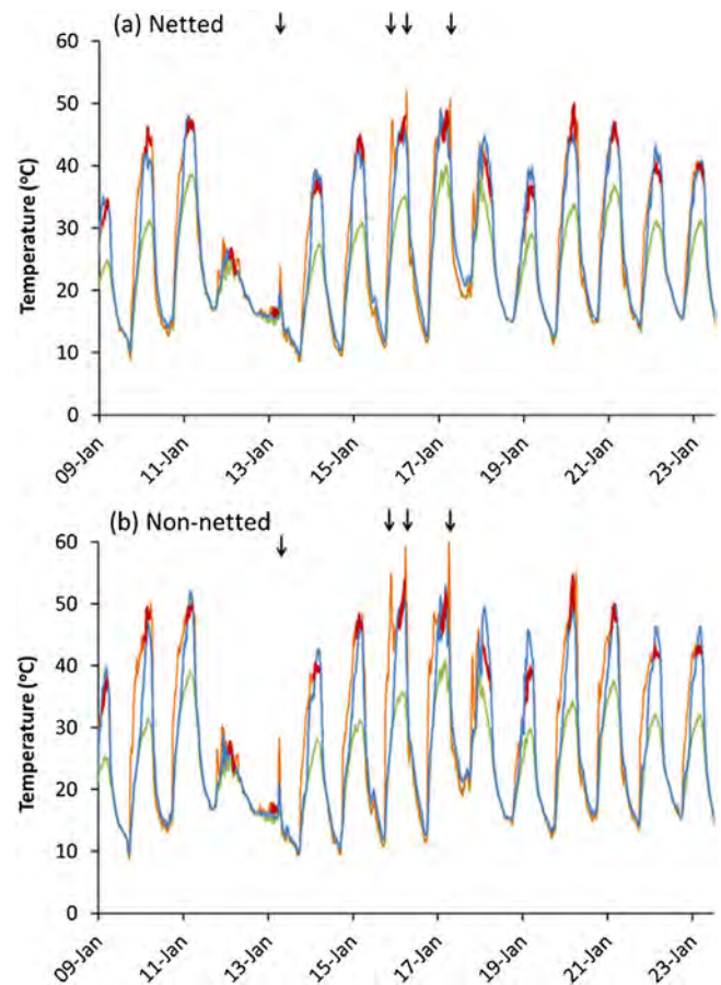
Fig. 1. Measured (blue) and simulated (red and orange) fruit surface temperature of the hottest face of sun-exposed fruit ( T_{fr,max} ) and orchard air temperature (green) at (a) netted, and (b) non-netted, with simulated T_{fr,max} calculated from wind speeds measured external to the orchard. Simulated temperatures are shown in red between 1400 and 1700 h, and orange at other times. Arrows show spikes in simulated values at times of low wind speed and high direct radiation before 1000 and after 1700 h. (For interpretation of the references to colour in this figure legend, the reader is referred to the web version of this article.)
