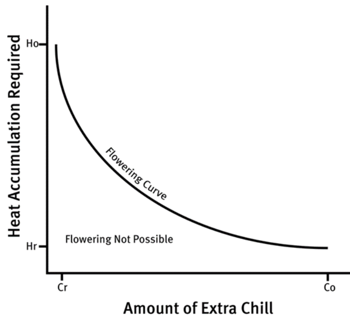
Figure 6. The Chill-Overlap Model for flowering in apple. Cr is minimum chill required for flowering, Co is the maximum additional chill that will reduce the heat requirement. Hr is the heat required when Co chill is accumulated, and Ho is the maximum possible heat requirement for flowering. (Redrawn from Darbyshire et al., 2016).
