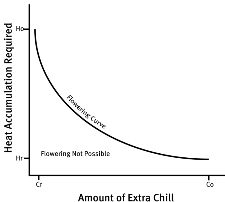
Figure 16 The Chill-Overlap Model. Cr is the chill required for flowering. Co is the maximum additional chill that will reduce the heat requirement. Hr is the heat required when Co chill is accumulated and Ho is the heat required when chill is an Cr (Redrawn from Darbyshire et al. 2016).
