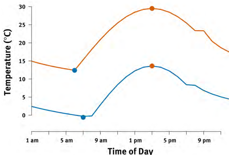
Figure 2 Examples of the use of the interpolation routine to convert daily maximum and minimum temperatures to hourly. The orange line is 21 December 2015 and the blue line is 21 June 2015 for Applethorpe. Dots indicate the maximum (orange) and minimum (blue) for each day that were used to generate the interpolated hourly data.
