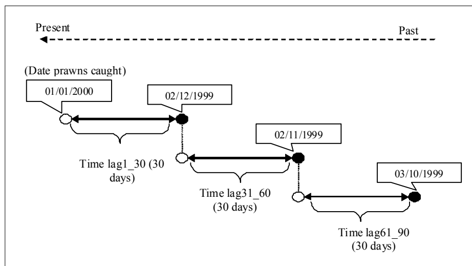
Figure 13-1. Illustrated process of how time lags were applied to the rainfall and flow data. Slightly different lags were applied to the temperature and SOI data. Diagram borrowed from Tanimoto et al. (2006).
