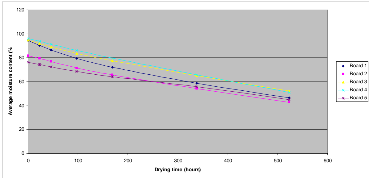
Figure 2.5.3. Average MC of average MC sample boards, messmate trial 3.
