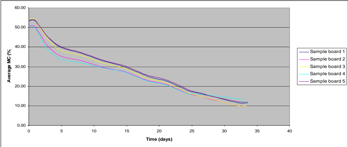
Figure 4.5.2. Moisture content of sample boards during drying
