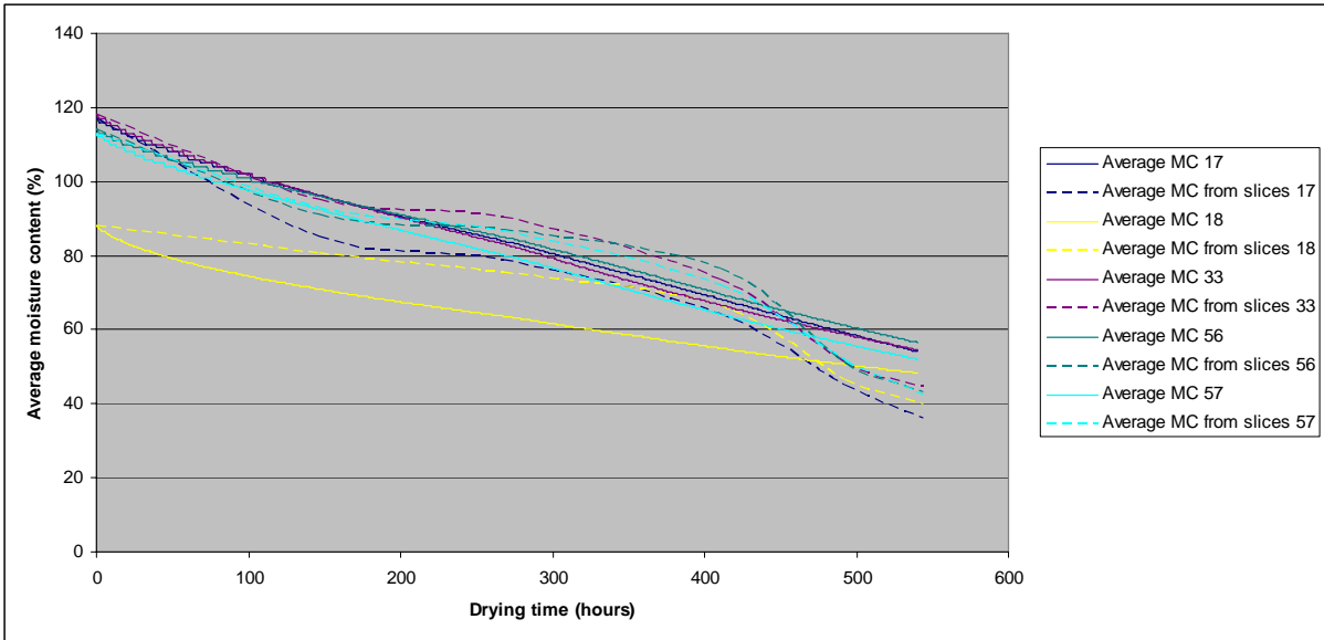
Figure 4.3.10. Average MC measured and predicted by model for DWTS sample boards
