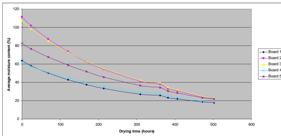
Figure 2.6.1. Average MC of sample boards, mountain ash trial.
