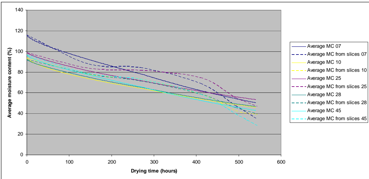
Figure 4.3.9. Average MC measured and predicted by model for Gould sample boards
