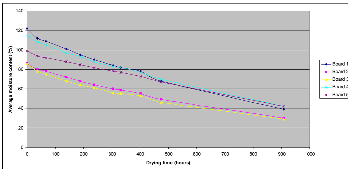
Figure 2.2.1. Average MC of sample boards, alpine ash trial.
