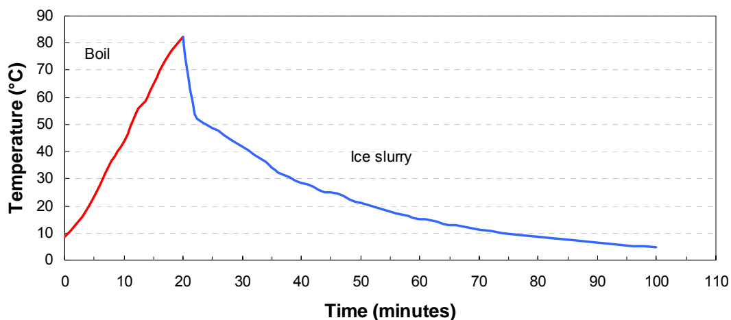
Figure 5.85. Core temperature of crabs during cooking and chilling.
