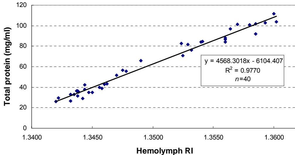
Figure 4.1 Standard curve of refractive index against total protein.
