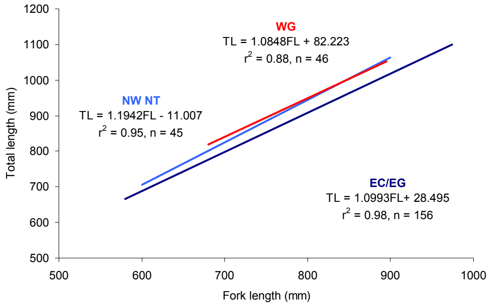
Figure 3.3. Total length (TL) – Fork length (FL) relationships among regions for female grey mackerel. The different regions are represented by the colours indicated (WG – red; NW NT – light blue; EC/EG – dark blue).
