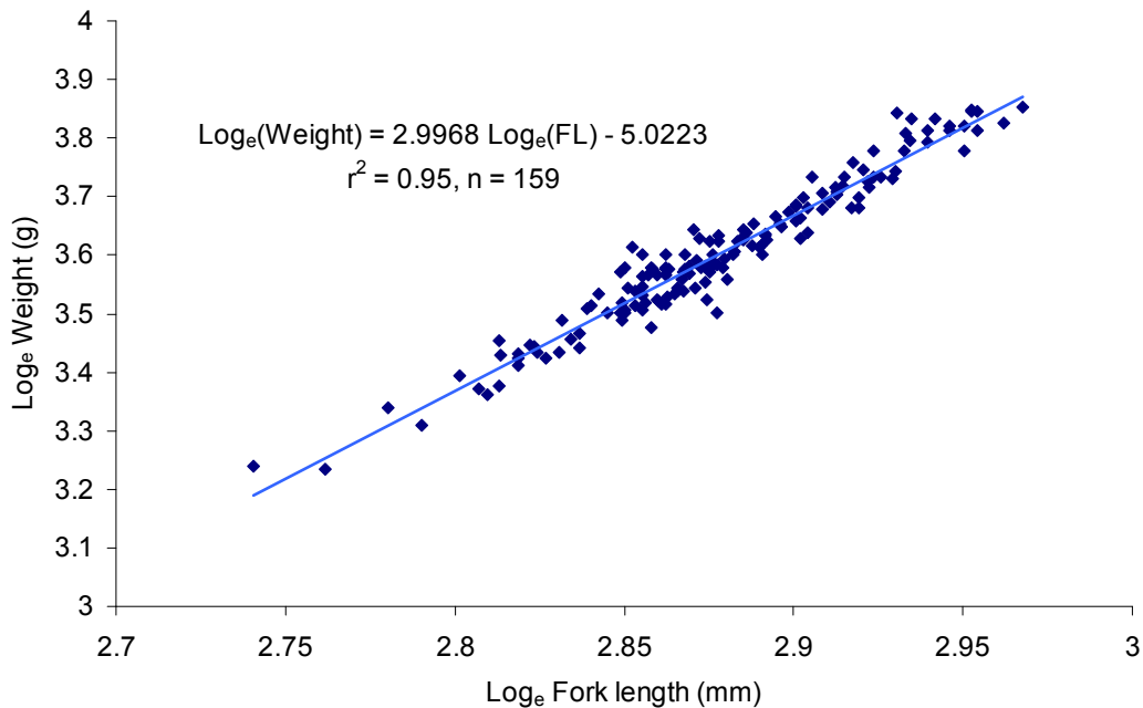
Figure 3.7. \log_e transformed Weight (g) – \log_e transformed Fork length (mm) relationship for grey mackerel (sex and regions combined).
