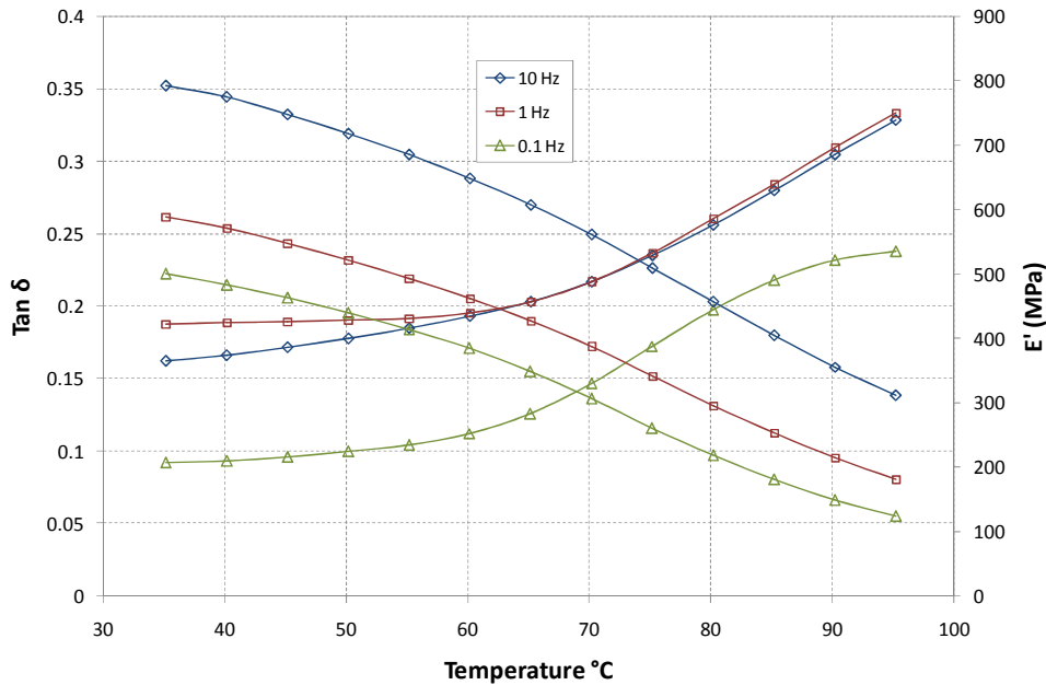
Figure 14. Development of the viscoelastic properties versus temperature of Eucalyptus marginata in the tangential direction, showing indeterminate glass transition temperature for every frequency.
