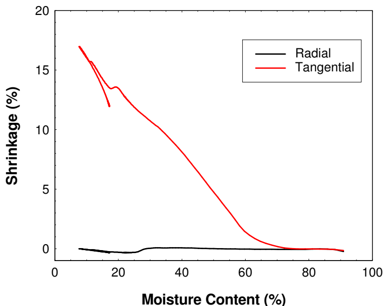
Figure 24. Tangential and longitudinal shrinkage of a Eucalyptus obliqua micro-sample
