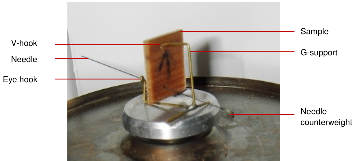
Figure 19. Sample support
