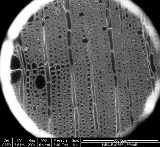
200 x magnification
