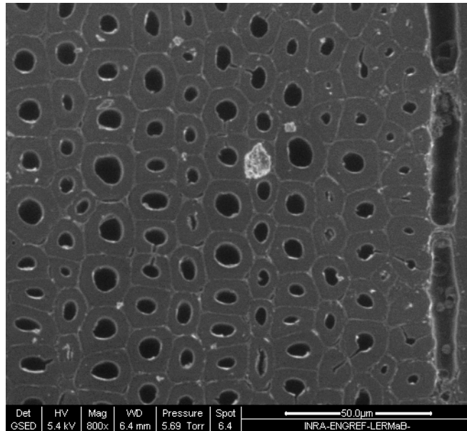
800 x magnification
