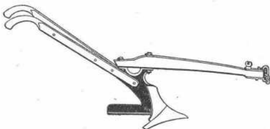
FIG. 1.—Plough Type of Peanut Digger
