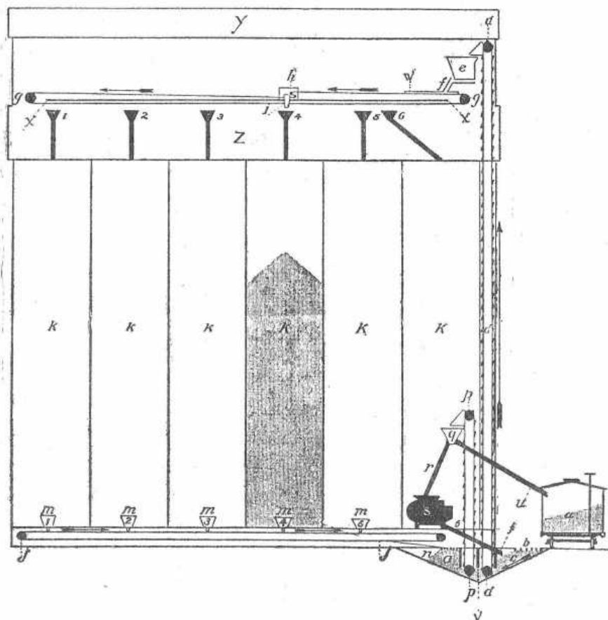
FIG. 3.—Diagram of an elevator. a , car with grain; b , grating over the hopper, c , hopper; d , pulleys carrying the endless band and elevator buckets; e , weighing-bin; f , w , delivery spout to grain belt; g , g , grain belt; h , zig zag, which is moveable back and forth on the track, x , x ; i , spout; k k k , bins or silos, to which the spouts, 1, 2, 3, 4, 5, 6, deliver grain; m m m , mouths of the bins or silos; l , l , carrying-belt delivery into the hopper, o , through the grating, n ; p , p , secondary elevator delivering to hopper, q , whence the grain may go to the cleaner, s , via r , or to the car, via u ; y , z , location of the roofs of the elevator.
