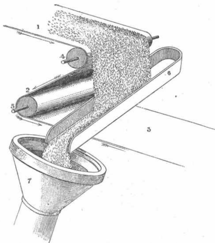
FIG. 4.—Diagram of a "zig-zag." The grain-carrying belt is shown at 1, 2, 3, and the direction of its motion is indicated by arrows; 4 and 5 are pulleys used to zig-zag the belt. The grain is shot into a trough, 6, which empties into a spout, 7, leading to a bin or elsewhere.
