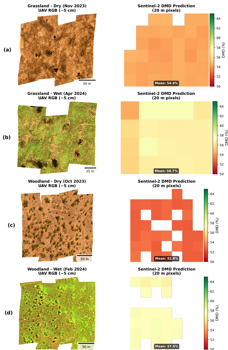
Figure 12. Multi-scale comparison of UAV hyperspectral RGB imagery (~5 cm) and Sentinel-2 satellite dry matter digestibility (DMD) predictions (20 m). Columns show: (1) UAV RGB imagery, (2) Sentinel-2 DMD predictions. Rows show two contrasting sites in dry and wet seasons: (a) grassland dry (November 2023), (b) grassland wet (April 2024), (c) woodland dry (October 2023), (d) woodland wet (February 2024).
