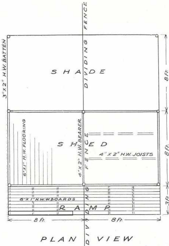
OPEN FRONTED SHELTER SHEDS FOR PIGS Being a Double Shed with a Dividing Fence Ramp in Front and Brush Shade at Back PLATE 16 (Fig. 13).
