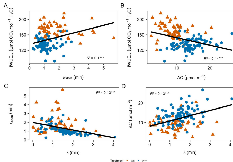
Fig. 2. Relationship between steady state water use efficiency and stomatal kinetic parameters in sorghum. Gas exchange measurements were taken during midday on the youngest fully expanded leaf. Steady state values were taken at 2000 \mu\text{mol m}^{-2} \text{s}^{-1} of light and 400 \mu\text{mol m}^{-2} \text{s}^{-1} \text{CO}_2 (see Materials and methods). The transition from low-to-high light was conducted from 100 to 2000 \mu\text{mol m}^{-2} \text{s}^{-1} , with the reverse for the high-to-low light. Calculation of stomatal kinetic parameters was done using modelling as described in Materials & methods. Each dot in the scatter is the mean for one genotype for that treatment ( n = 3 ). Correlation coefficients ( R^2 ) are the result of a Pearson correlation test. ***, P < 0.001 . Blue dots are for well-watered, red for water-stressed. (A) Steady-state iWUE ( \text{iWUE}_{\text{ss}} ) vs. time-constant of stomatal opening ( k_{\text{open}} ). (B) \text{iWUE}_{\text{ss}} vs. Forgone photosynthesis ( \Delta C ). (C) k_{\text{open}} vs. time-lag constant of stomatal response ( \lambda ). (D) \Delta C vs. \lambda . Standard error can be found in Tables S4 and S5 . (NB, faster stomata is defined as low k_{\text{open}} ).
