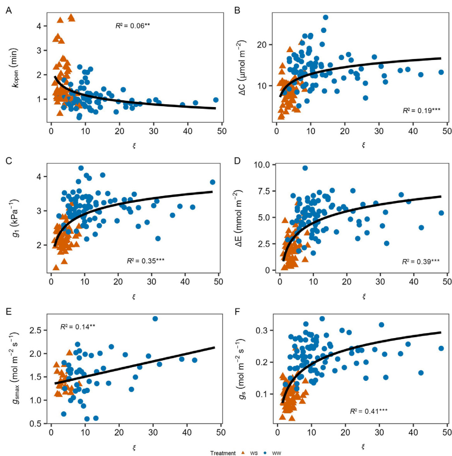
Fig. 4. Relationship between hydric behavior and stomatal behavior in sorghum. Gas exchange measurements were taken during midday on the youngest fully expanded leaf. Steady state values were taken at 2000 \mu\text{mol m}^{-2} \text{s}^{-1} of light and 400 \mu\text{mol m}^{-2} \text{s}^{-1} \text{CO}_2 (see Materials and methods). Transition from low-to-high light was conducted from 100 to 2000 \mu\text{mol m}^{-2} \text{s}^{-1} , with the reverse for the high-to-low light. Calculation of stomatal kinetic parameters was done using modelling as described in Materials and Methods. Degree of anisohyry was calculated as the ratio of midday to pre-dawn leaf water potentials. For pre-dawn water potential, leaves from lower down the canopy were sampled into a plastic bag in a coolbox and taken to the lab. For midday water potential, the leaf adjacent to that used for gas exchange was sampled into a wet paper bag and into a coolbox, transported to the lab and measured within 2 h. Midday leaves were sampled during the same diurnal gas exchange period on sunny days. Each dot in the scatter is the mean for one genotype for that treatment ( n = 3 ). Correlation coefficients ( R^2 ) are the result of a Pearson correlation test. **, P < 0.01 ; ***, P < 0.0001 , or from the exponential fit of the model. (A) Time-constant of stomatal opening ( k_{\text{open}} ) vs. degree of anisohyry. (B) Forgone photosynthesis ( \Delta C ) vs. degree of anisohyry. (C) Slope coefficient of stomatal response to photosynthesis and VPD ( g_1 ) vs. degree of anisohyry. (D) Excess transpiration ( \Delta E ) vs. degree of anisohyry. (E) Anatomical maximum stomatal conductance ( g_{\text{smax}} ) vs. degree of anisohyry. (F) Stomatal conductance ( g_s ) vs. degree of anisohyry. Standard error can be found in Tables S4 and S5 .
