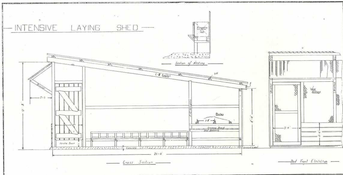
PLATE 103.—SHOWING END SECTION AND PART FRONT ELEVATION OF INTENSIVE LAYING SHED.
