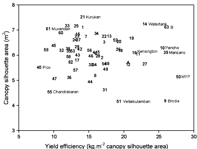
Fig. 1. Relationship between tree size (canopy silhouette area) and yield efficiency of 'Kensington Pride' mango on 64 rootstocks. Rootstock names of most interest are indicated following the plotted accession numbers (as per Table 1).
