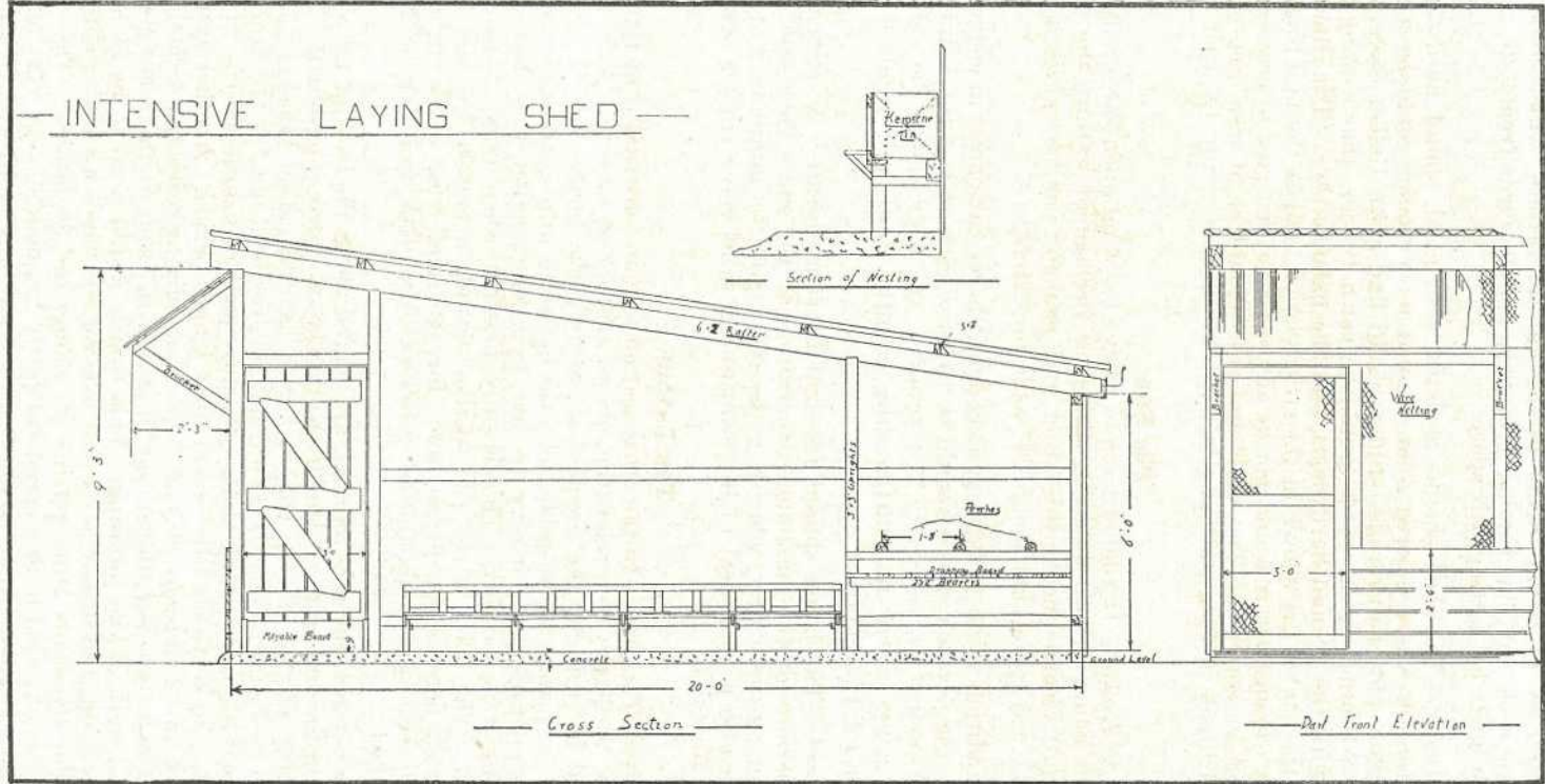
PLATE 42.—SHOWING END SECTION AND PART FRONT ELEVATION OF INTENSIVE LAYING SHED.
