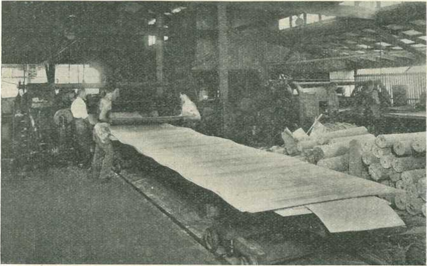
PLATE 59.—PEELING HOOP PINE LOGS ON ROTARY LATHE.
