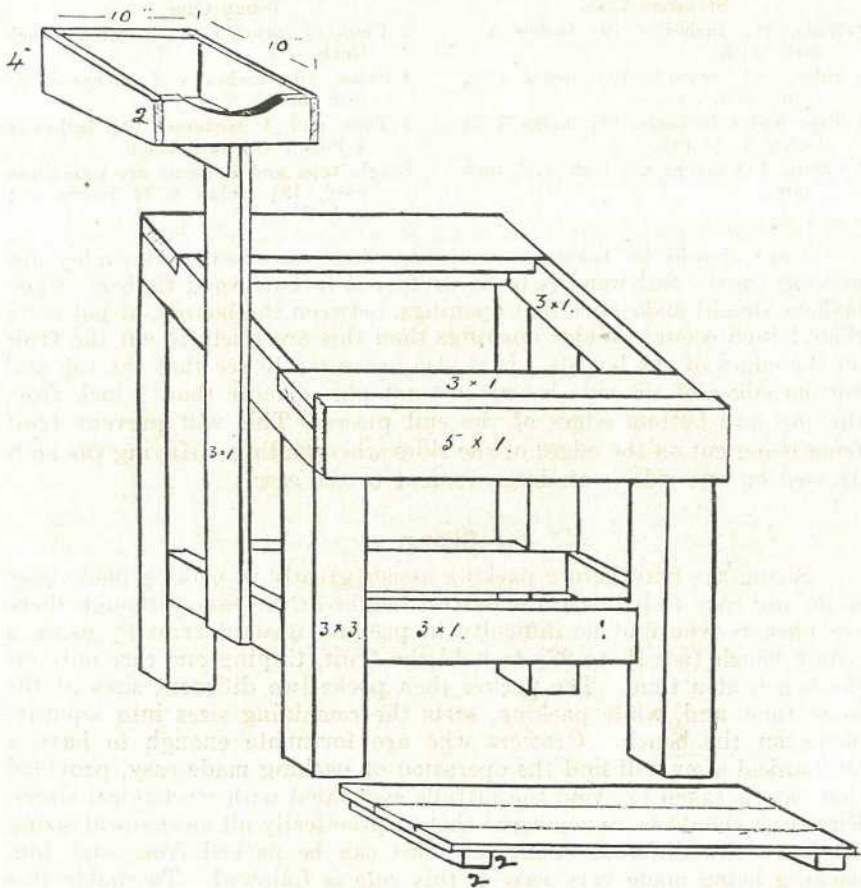
PLATE 24.—PACKING STAND.
