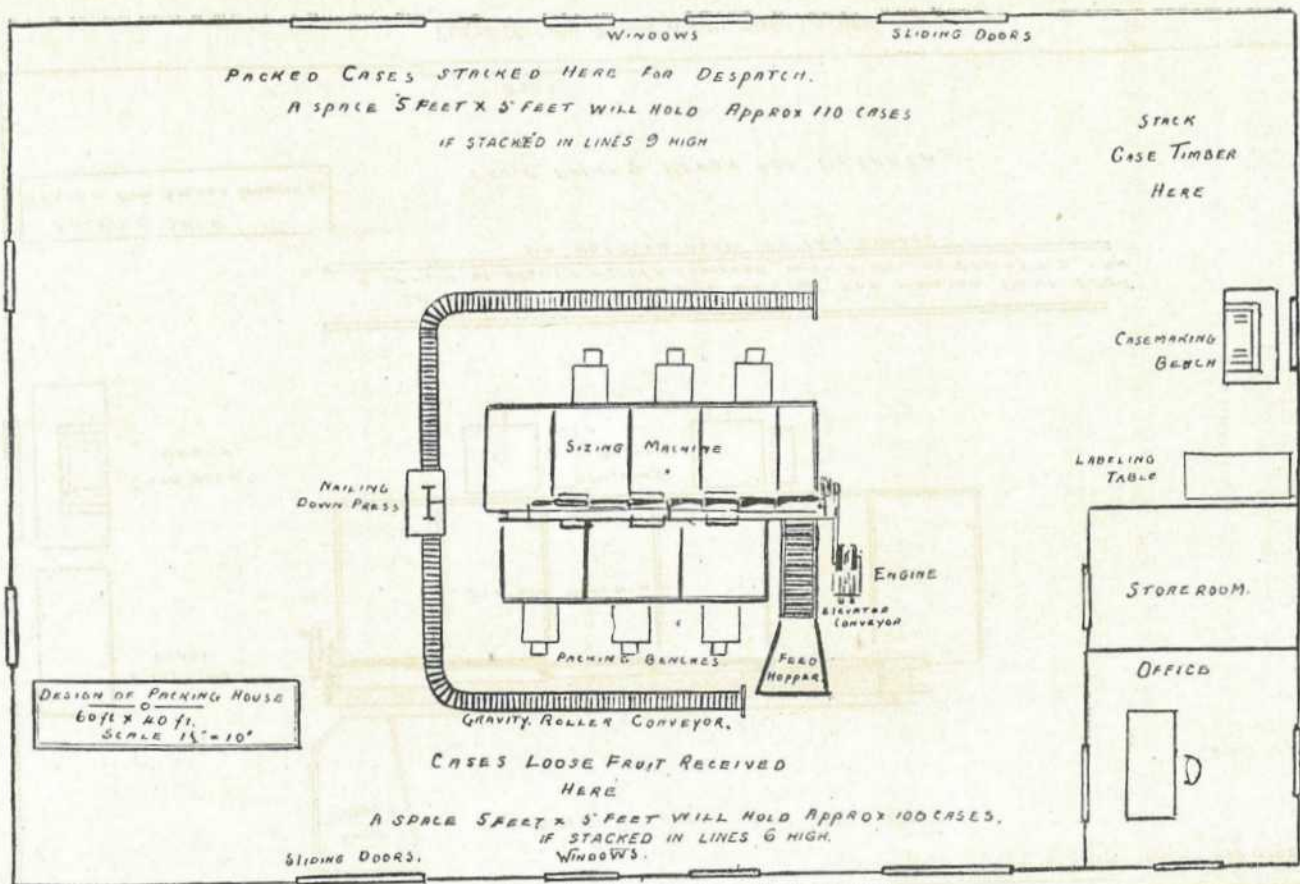
PLATE 19 (Fig. 1).—PACKING SHED LAYOUT.
