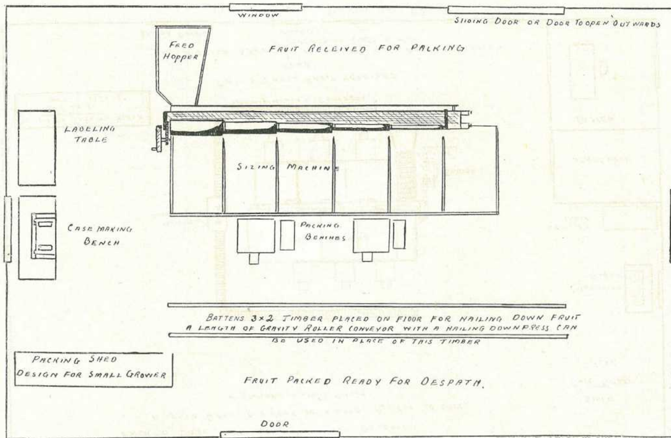
PLATE 20 (Fig. 2).—PACKING SHED LAYOUT,
