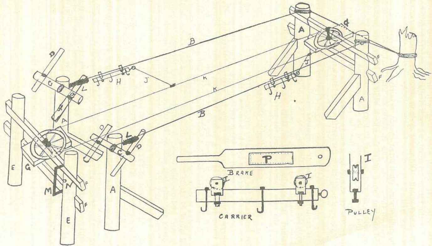
Plate 57. SKETCH SHOWING DETAILS OF WIREWAY CONSTRUCTION.
