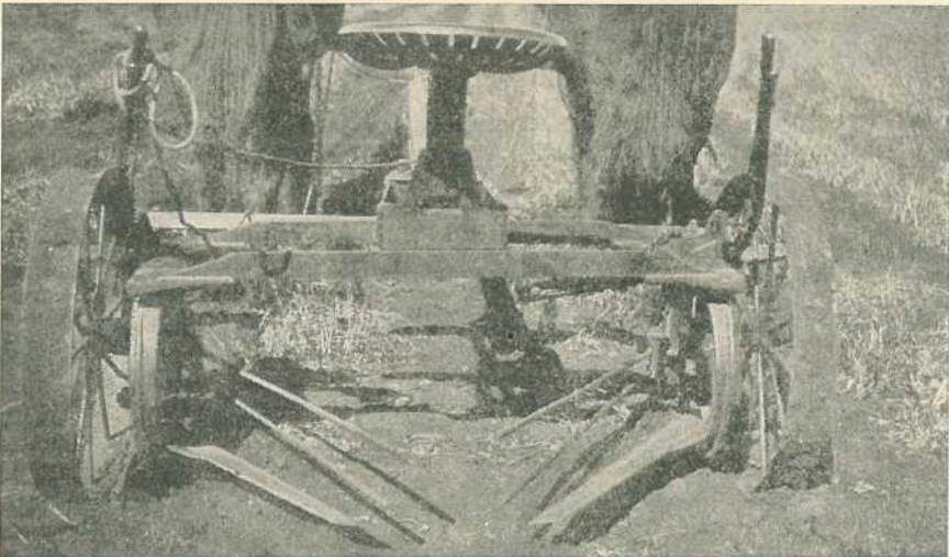
Plate 55. A close-up view of a two-row bean cutter, showing cutting blades and guide rods for placing bean plants into a single windrow.
