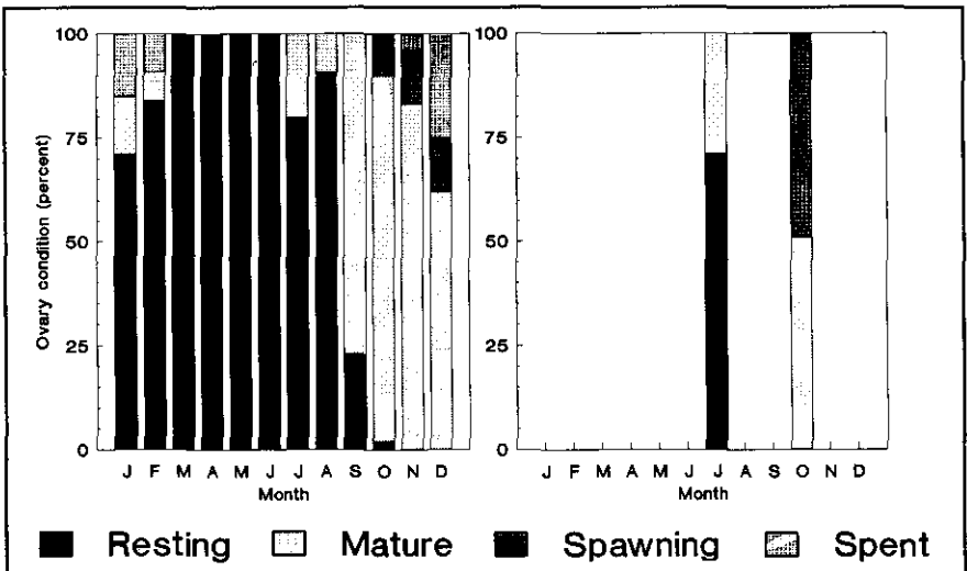
Fig. 2. Seasonal variation of grouped ovary macroscopic stages from east coast (left) and northern Australian (right; that is, Morington Island and Torres Strait) stocks of S. commerson .
