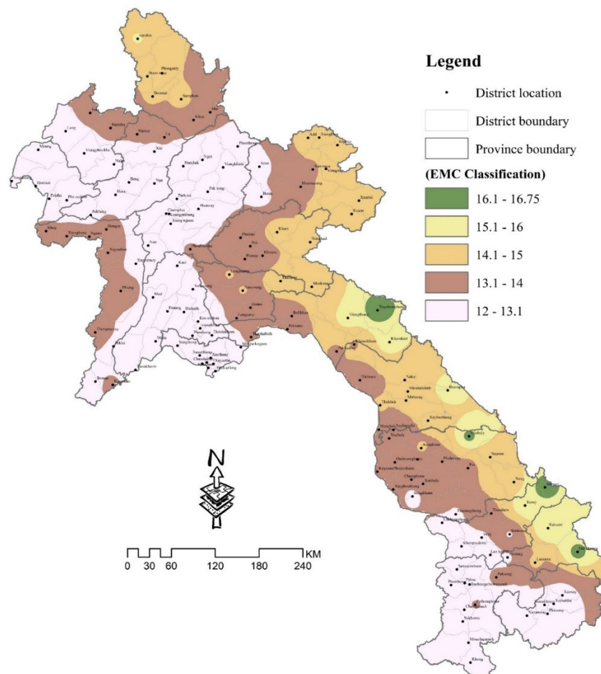
Figure 1: Equilibrium moisture content map of Lao districts
