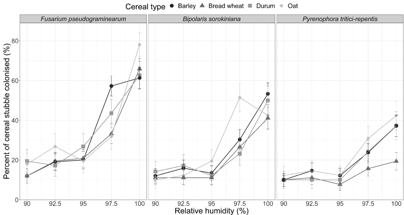
Fig. 1 Colonisation of stubble from four cereal species by three cereal pathogens, as a percentage (%) of cereal stubble height colonised after seven days, under differing relative humidity regimes. Error bars represent approximate standard error of the mean
