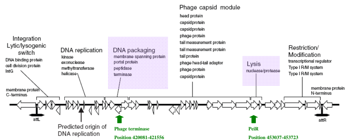
Figure 1. Predicted functional modules and gene structure for \phi mru, the prophage present within the Methanobrevibacter ruminantium M1 sequence (Accession NC_013790.1), showing the completed chromosome position of the PeiR and terminase large subunit genes (highlighted) used for PCR primer design (Figure adapted from Attwood et al. 2008).
